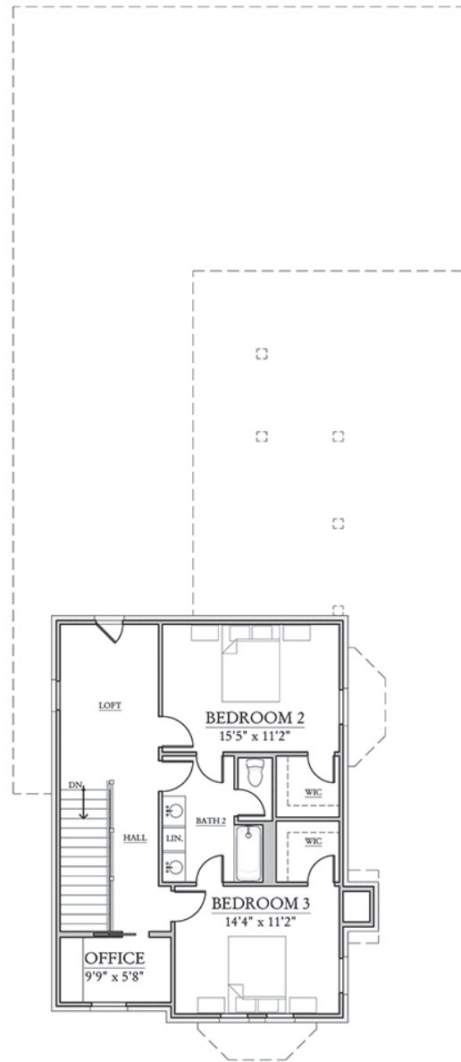
SECOND FLOOR
